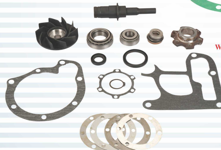
TATA 497/697 Part No. 2525-2099-0111 FOR WP ASSY. 2525-2010-0141
