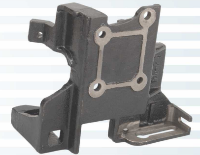
SUBROS CMB Part No. 646260 - 4361-O-L
